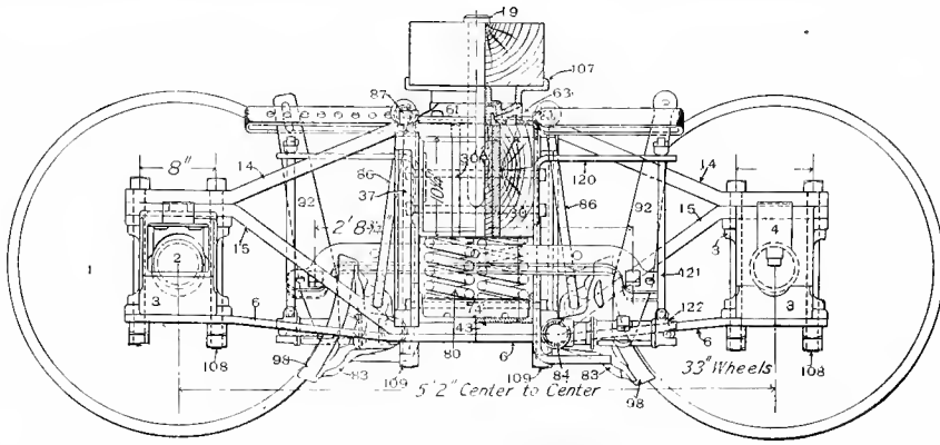
Fig. 4580 Sectional Side Elevation.
